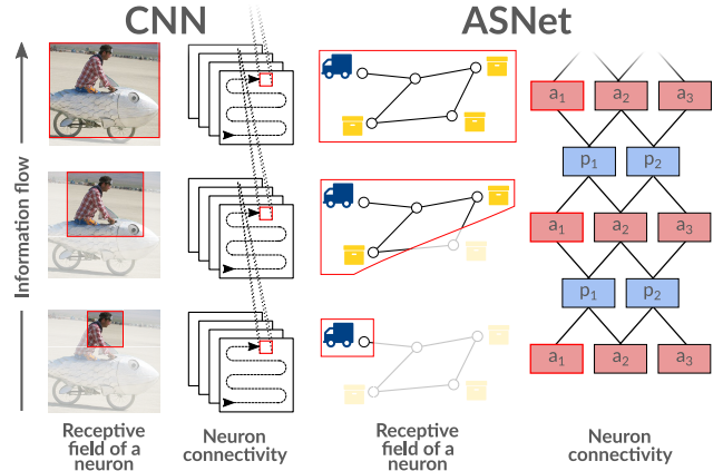
Figure 1: In a CNN, successive convolutions grow the receptive field of a neuron at higher layers; analogously for ASNet, a neuron for a particular action a or proposition p sees a larger portion of the current state at higher layers.
